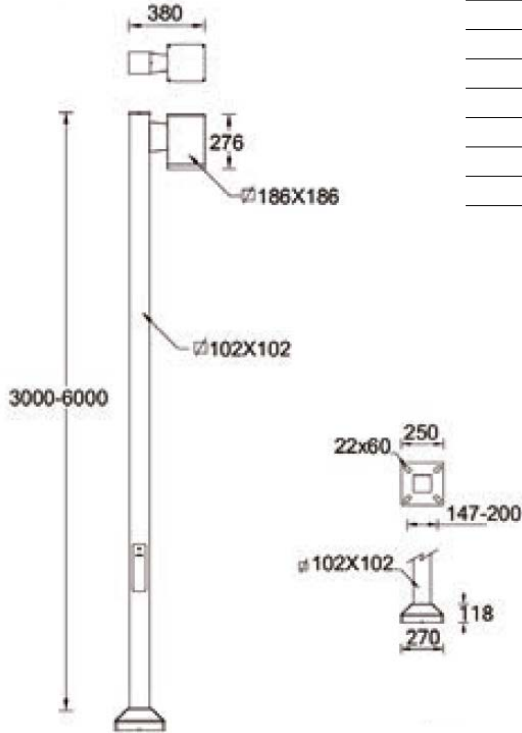
ALUMINIUM POST MOUNTING DETAIL
