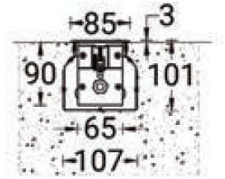
MOUNTING DETAIL
